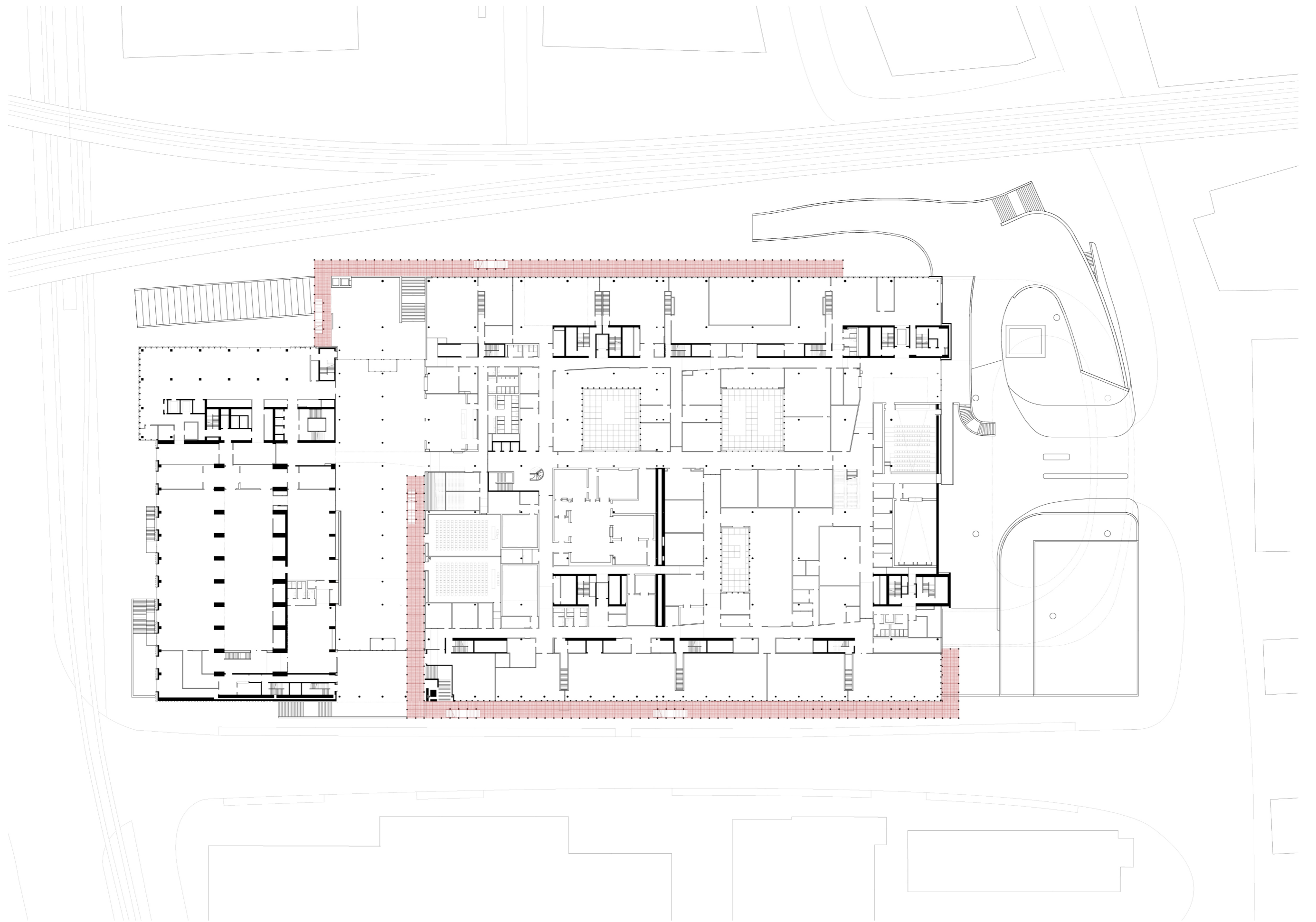
Ground Floor 02
