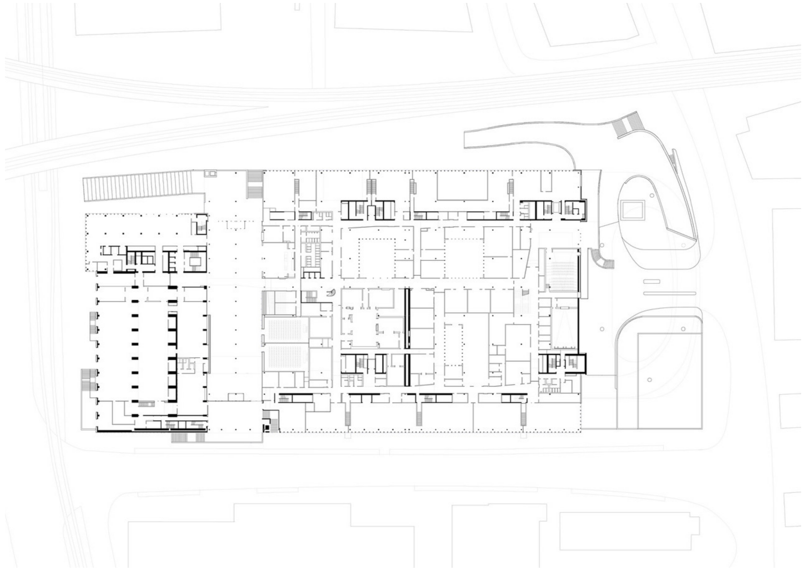
Ground Floor 01
